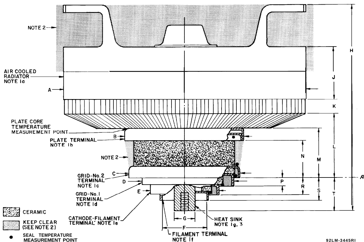
Figure 6 - Dimensional Outline
