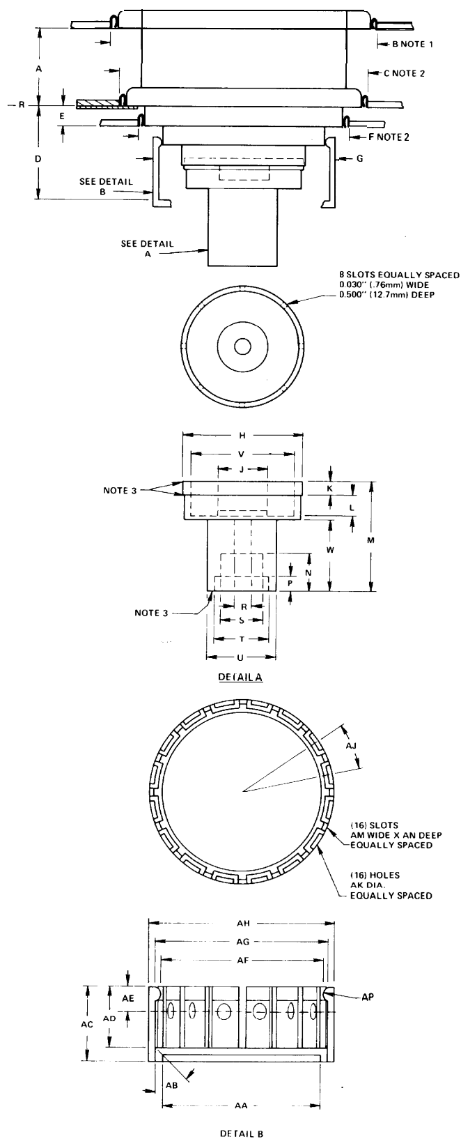
Figure 5 - Preferred Mounting Arrangement
