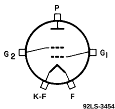
Figure 7 - Terminal Diagram
